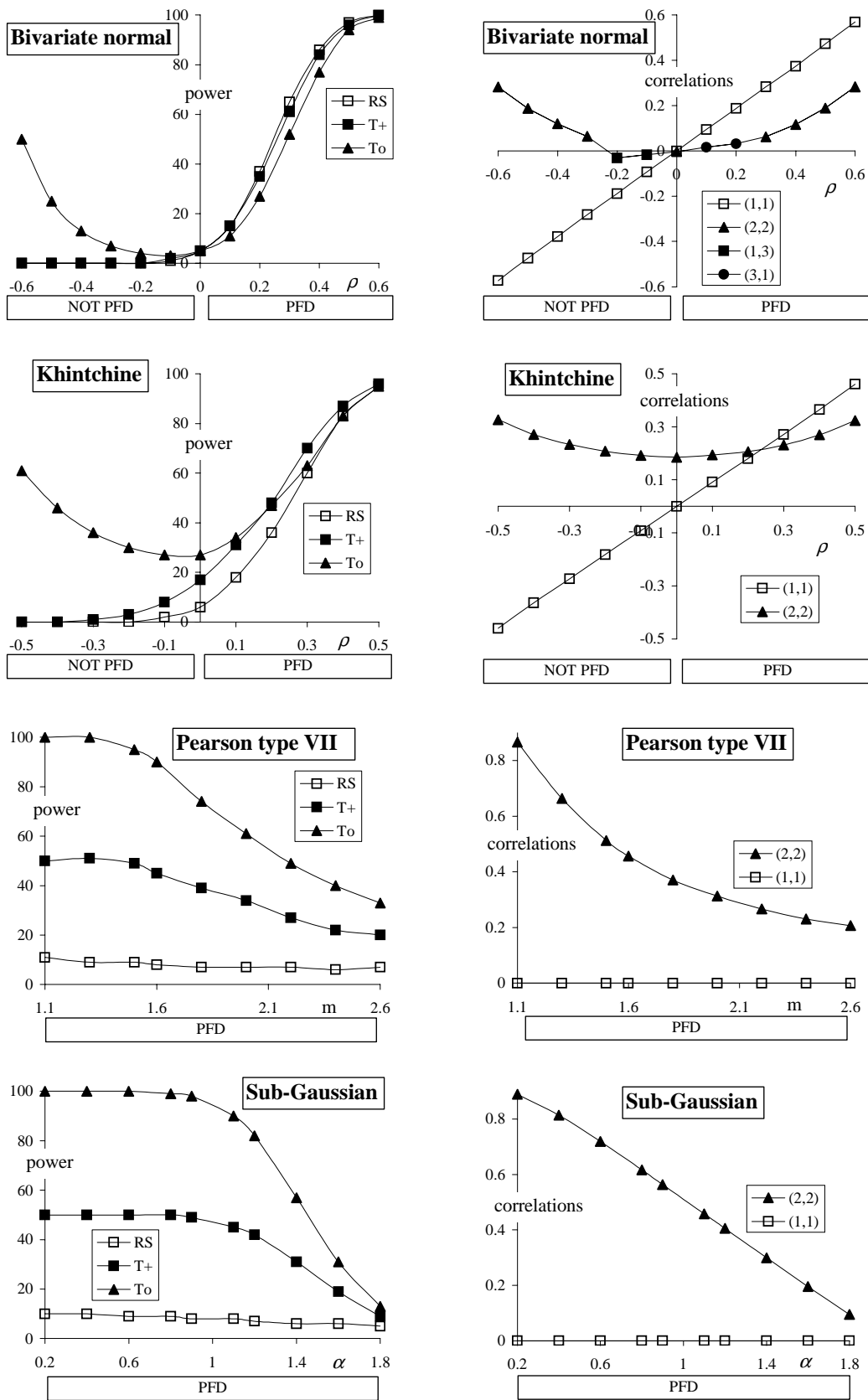
Figure 3. The simulated powers of 3 tests and the simulated correlation \hat{c}_{11} together with the (next) most important simulated correlation \hat{c}_{rs} at distributions d6 - d9 .
